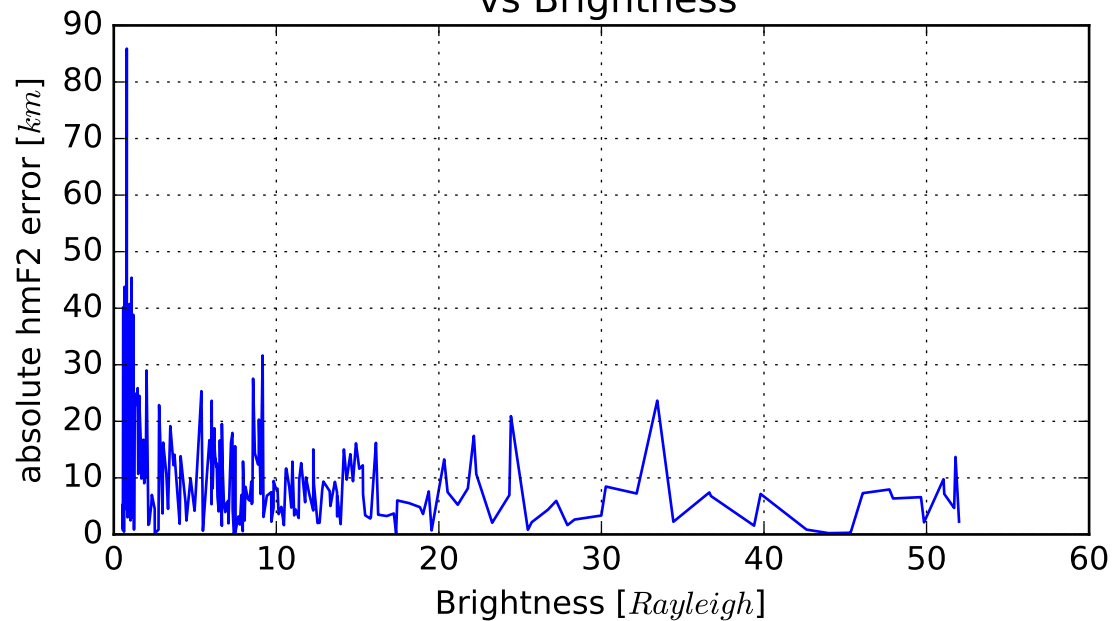
Absolute hmF2 error vs Brightness
