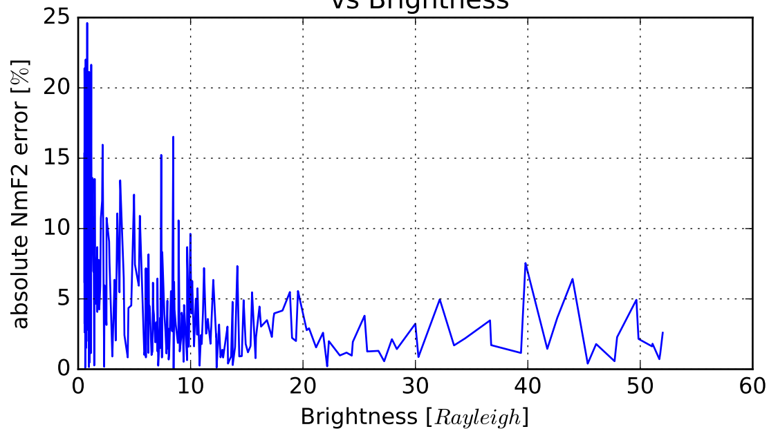
Absolute NmF2 error vs Brightness
