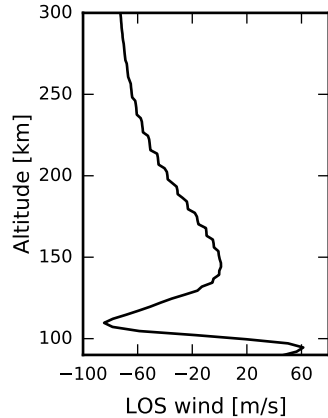
Retrieved Wind
