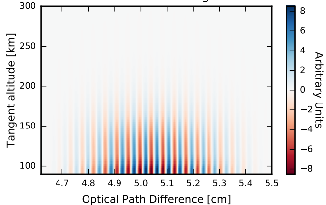
Calibrated Interferogram
